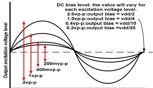
Figure 44. Output Excitation Voltage Levels and Bias Values
