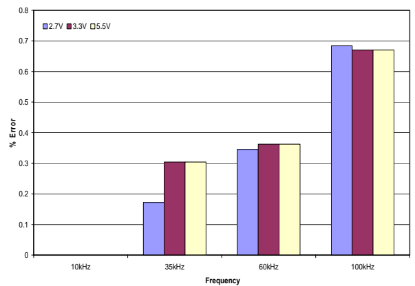
Figure 27. Impedance Error over 10 kHz to 100 kHz Range, Gain Factor @ 10 kHz
